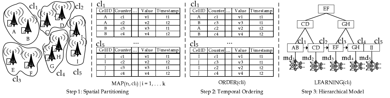
Fig. 4. The conceptual steps of the proposed TBD-DP construction algorithm.
